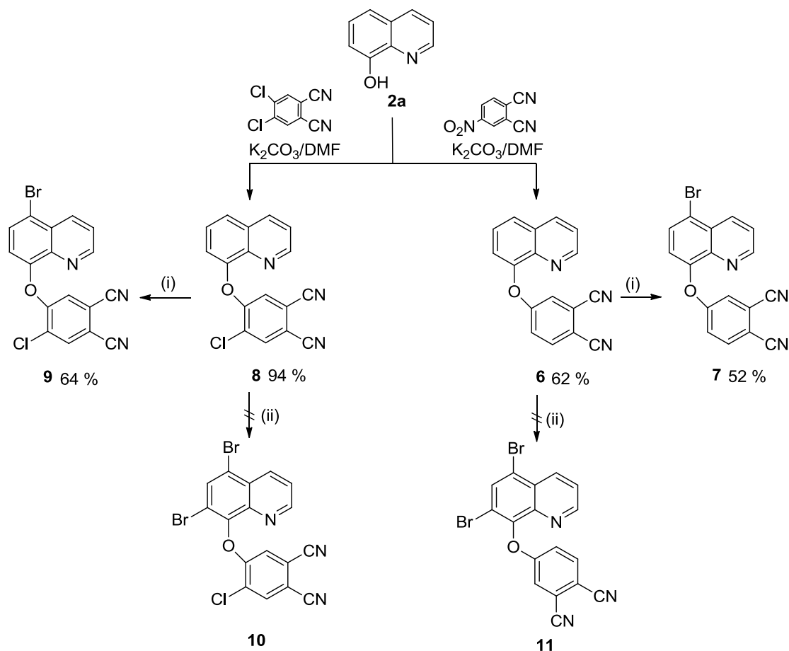
Figure 4. Synthesis and bromination of novel phthalonitrile derivatives ( 6 and 8 ) Reagents and conditions. (i) Br_2 (1 eq), CH_3CN , 0^\circ C , 34 h; (ii) Br_2 (2 eq), CH_3CN , 0^\circ C , 34 h.
