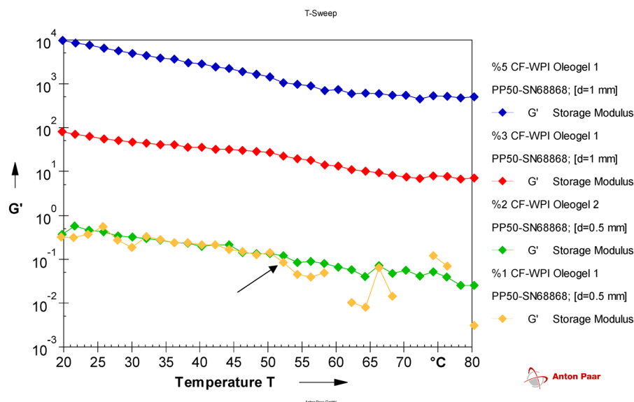
Figure 4 Temperature sweep test of oleogels.
