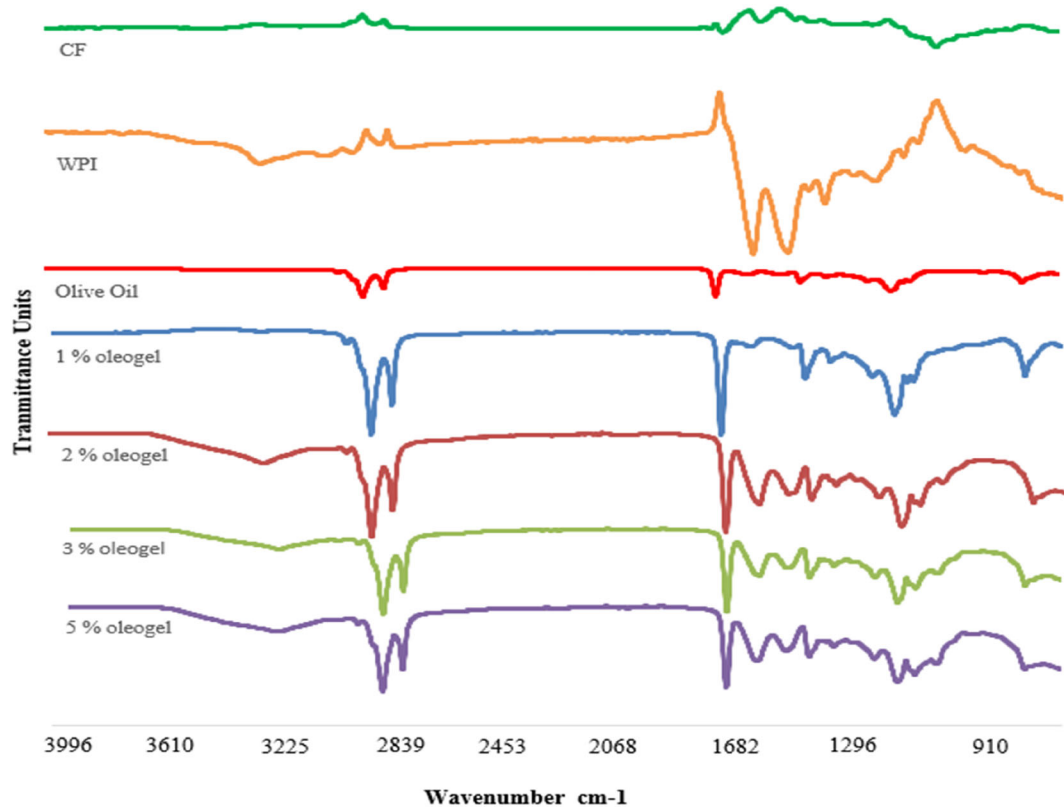
Figure 5 FTIR spectra of the CF, WPI, olive oil and oleogels.
