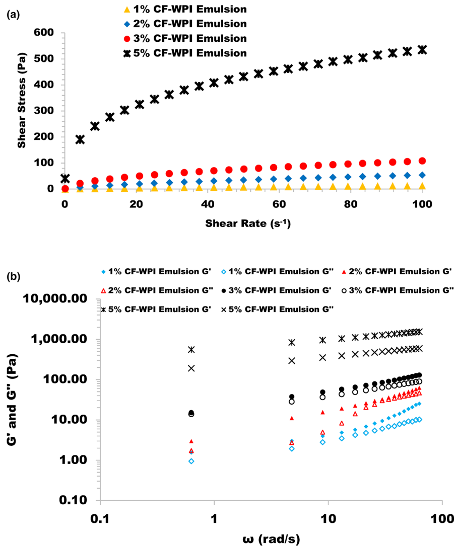
Figure 1 Steady shear (a) and dynamic rheological (b) properties of the emulsions.
