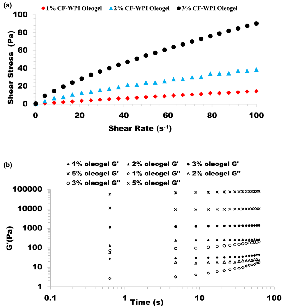
Figure 3 Steady shear (a) and dynamic rheological (b) properties of the oleogels.
