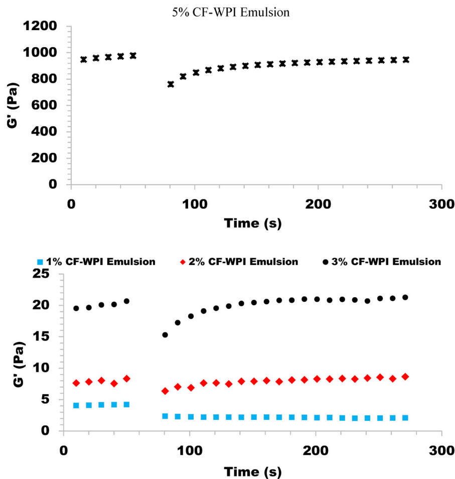
Figure 2 3-ITT rheological properties of emulsion.
