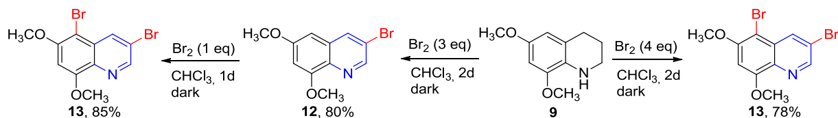
Scheme 5. Bromination of 6,8-dimethoxide 9 .
