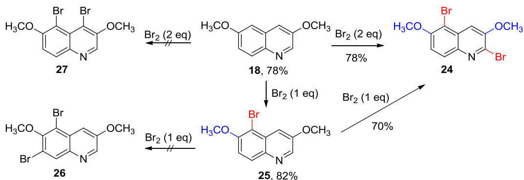
Scheme 8. Bromination of dimethoxide 18 and preparation of dibromide 24 .
