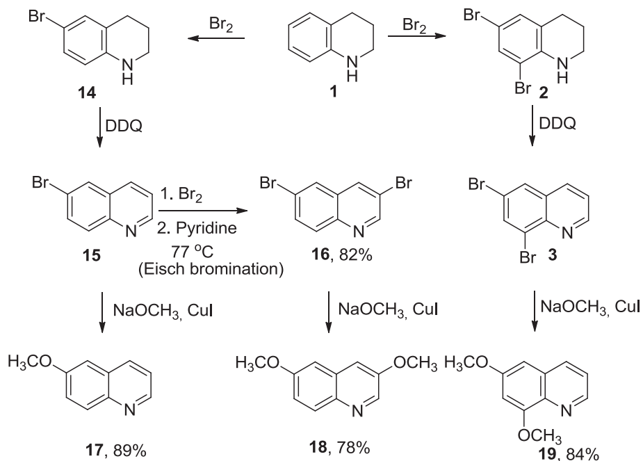
Scheme 6. Synthesis of starting compounds 17–19 .
