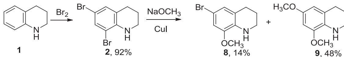
Scheme 3. Preparation of starting materials.
