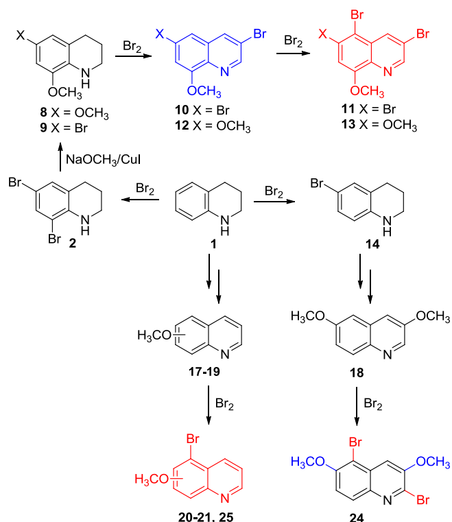
Scheme 9. General overview of bromination methods for methoxy quinolines/tetrahydroquinolines.
