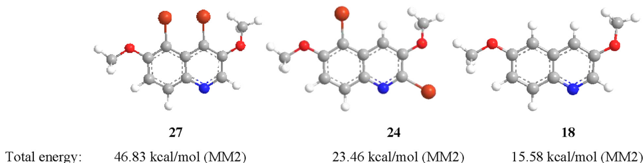
Fig. 1. 3D Structures of 18 , 27 , 24 and their total energies.
