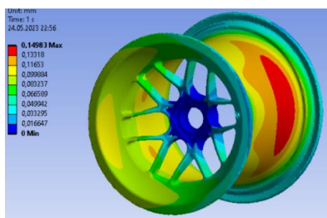
Figure 5. Total deformation result for Mg AZ80
