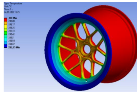
Figure 10. Thermal analysis results for carbon fiber
