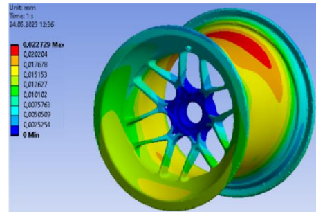
Figure 7. Total deformation result for carbon fiber
