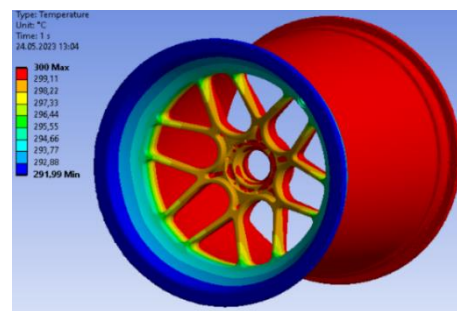
Figure 9. Thermal analysis result for Al 6061-T6
