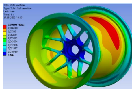
Figure 6. Total deformation result for Al 6061-T6
