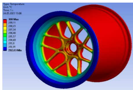
Figure 8. Thermal analysis result for Mg AZ80
