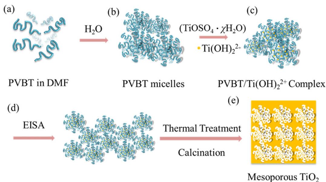
Scheme 1. Schematic representation of the mechanism of formation of a mesoporous \text{TiO}_2 film.
