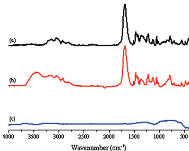
Figure 1. FTIR spectra of (a) pure PVBT, (b) PVBT/Ti(OH) 2+ complex obtained after heating at 170 °C, and (c) mesoporous TiO 2 obtained after calcination at 450 °C.
