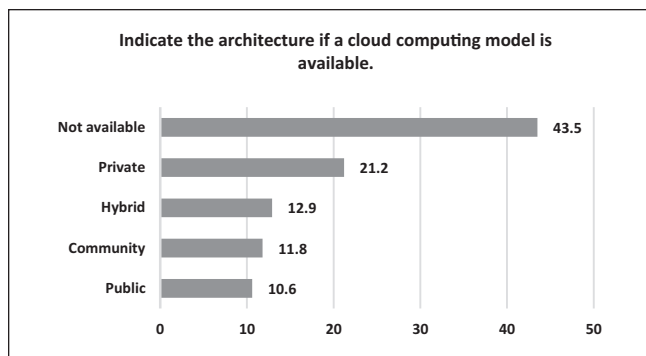
Figure 5. Architecture status.
