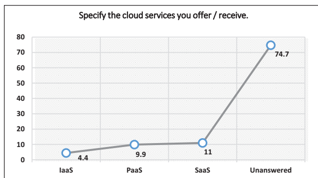
Figure 6. Cloud services.
