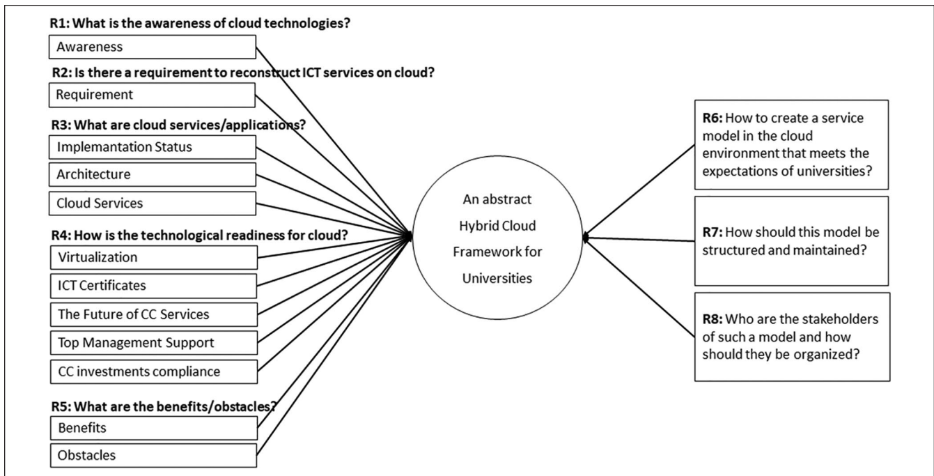
Figure 1. Research questions.
