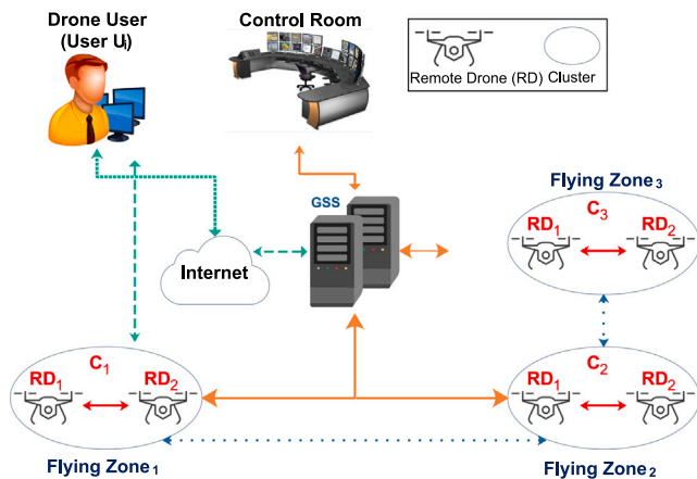
Fig. 1. IoD communication architecture.
