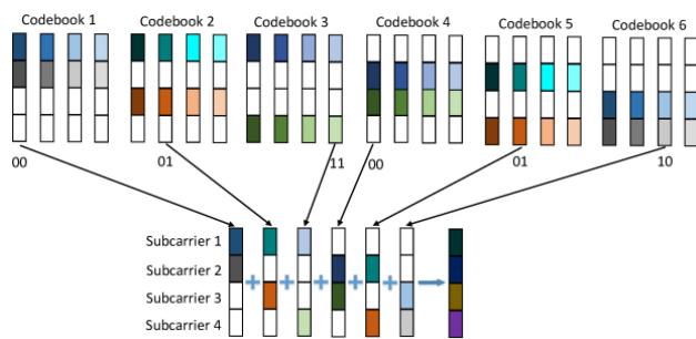
FIGURE 13. SCMA Codebook.
