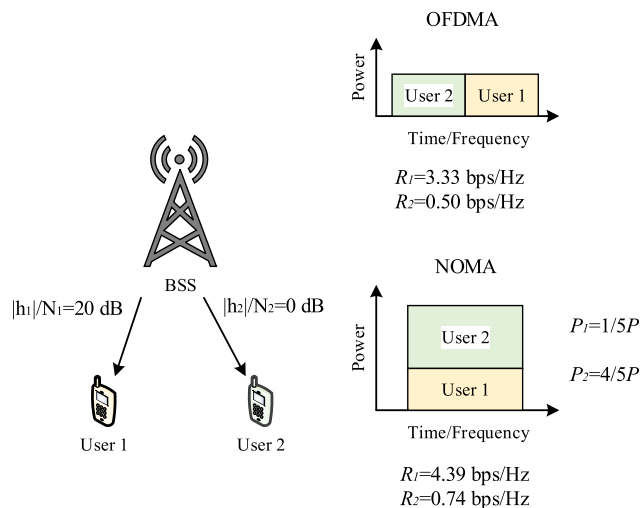
FIGURE 8. OFDMA vs NOMA.
