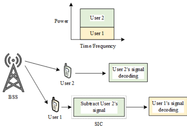
FIGURE 6. NOMA workflow.
