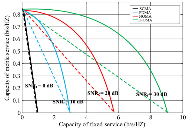
FIGURE 16. A collective figure showing the capacity of SCMA, FDMA, NOMA, D-OMA.
