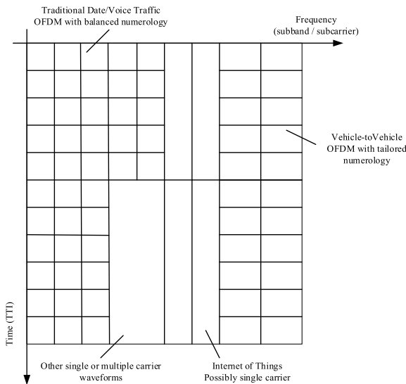
FIGURE 3. Example of OFDMA.
