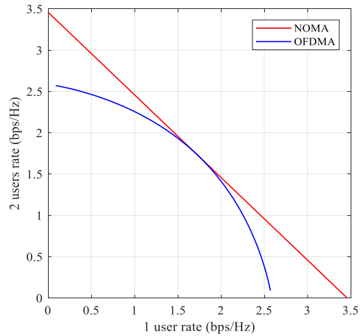
FIGURE 9. Bit rate per user (NOMA and OFDMA).
