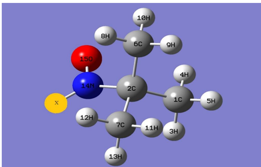
Fig. 1. Optimized structures of 2-methyl-2-nitrosopropane spin adducts (X; H, OH, SO 3 , CH 3 , CCl 3 C 6 H 5 ).
